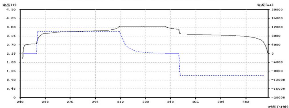
38120S 10AH 1C Charge and Discharge Curve
