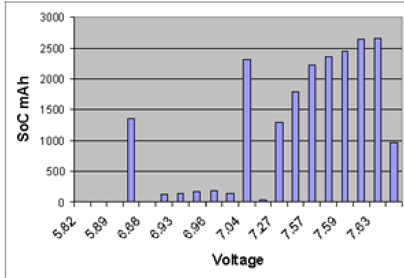
Battery pack from Silver Insight 150K on pack
