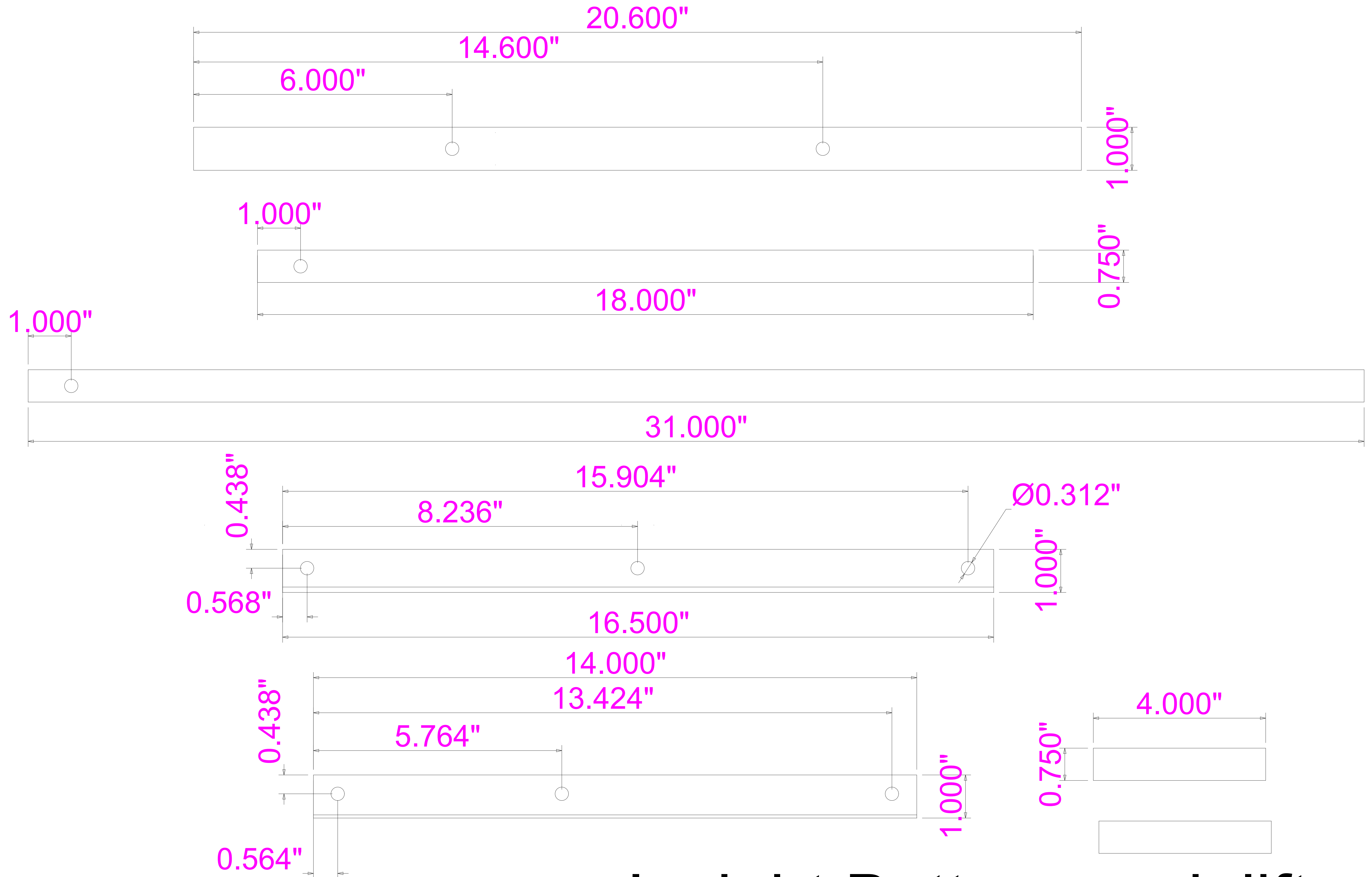
Insight Battery pack lifter
